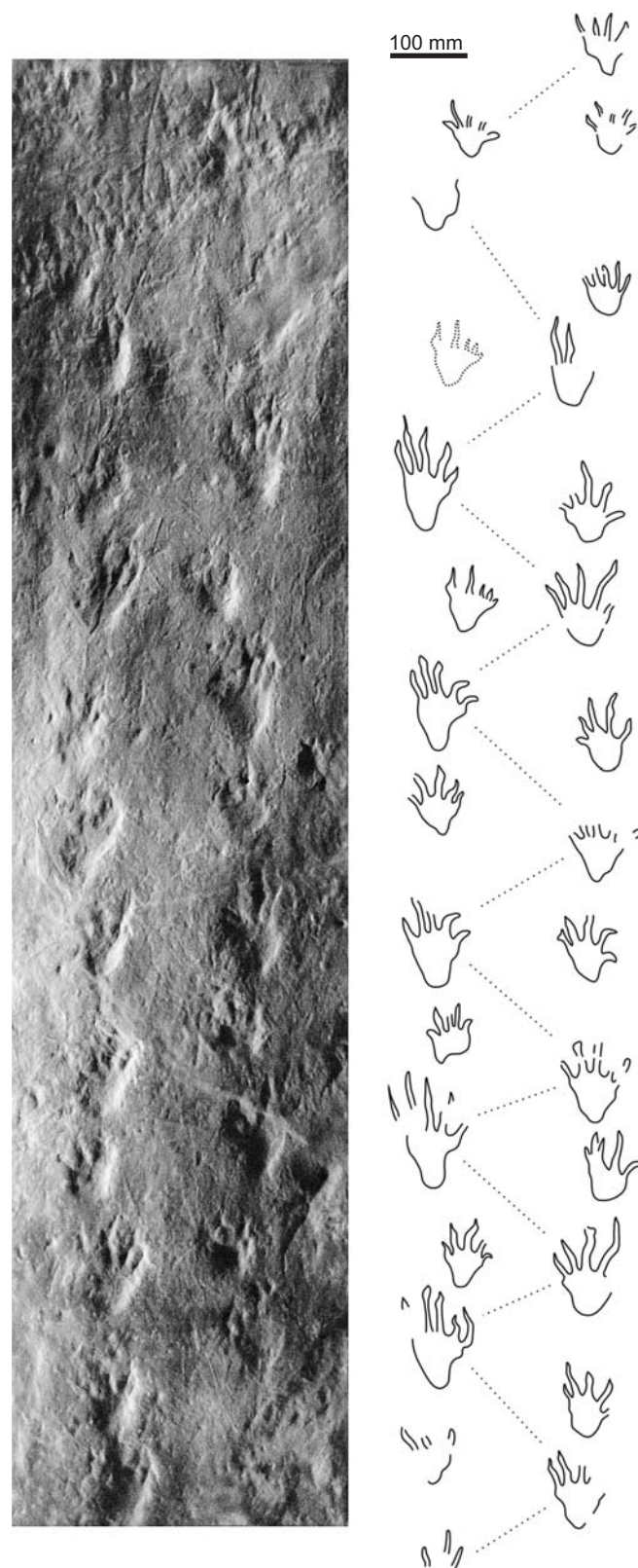
Fig. 5. Tetrapod footprints of Dimetropus sp. indet., from the Late Carboniferous Bochum Formation, Ruhr area, Germany. The photograph shows one of the two plaster casts of the trackway (DBM 060003357001); it is restricted to the most detailed tracks excluding faint imprints at the beginning and end of the trackway. The outline drawing illustrates the complete trackway as preserved on the five separated blocks of the original material.
