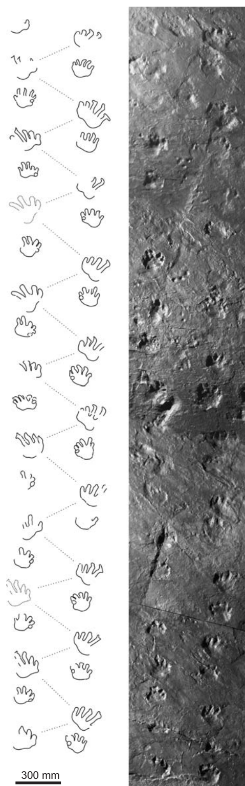
Fig. 2. Tetrapod footprints of Ichniotherium praesidentis (Schmidt, 1956) from the Late Carboniferous Bochum Formation, Ruhr area, Germany, represented by the longest and best preserved trackway of the holotype. Photograph and drawing are based on the four-part resin replica (DBM 060003309001 to DBM 060003309004). Note: the first two imprints are erroneously replicated twice and therefore not shown in the outline drawing. Dotted zigzag line links the pes imprints, and dotted track outlines indicate the position of imprints, which are reasoned from the step cycle but not preserved on the cast.
