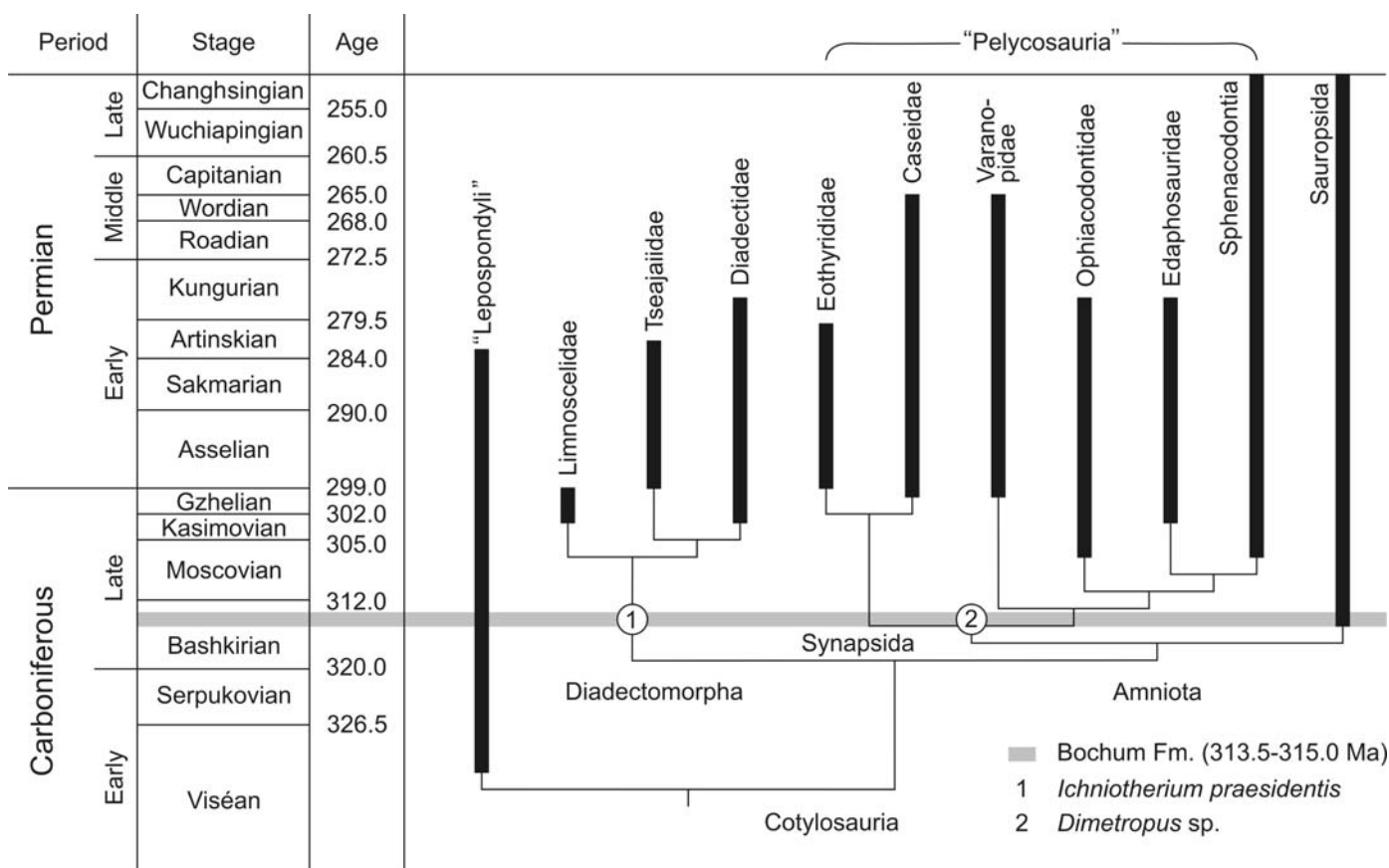
Fig. 8. Stratocladogram of tetrapod phylogeny. Although extending the known body fossil record, the stratigraphic position of the diadectomorph and synapsid footprints from the Bochum Formation of western Germany fits well the phylogenetic pattern. Black bars indicate the known record of skeletal remains (Reisz 1986; Kissel and Reisz 2004a, b). Cladogram topology and minimum times of divergence are based on Kissel and Reisz (2004a, b), Müller and Reisz (2004), and Reisz (2007). The chronostratigraphic scale is adopted from Menning (2005).
